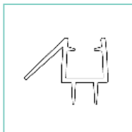
10mm Horizontal Glass Flap PGFH
